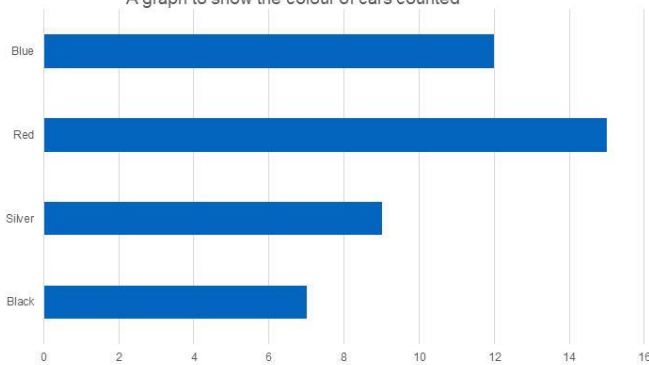
A graph to show the colour of cars counted
